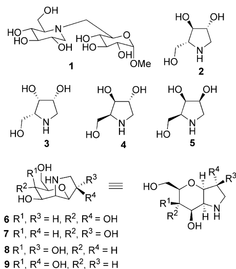
Figure 1. Piperidine- and pyrrolidine-based iminosugars.
