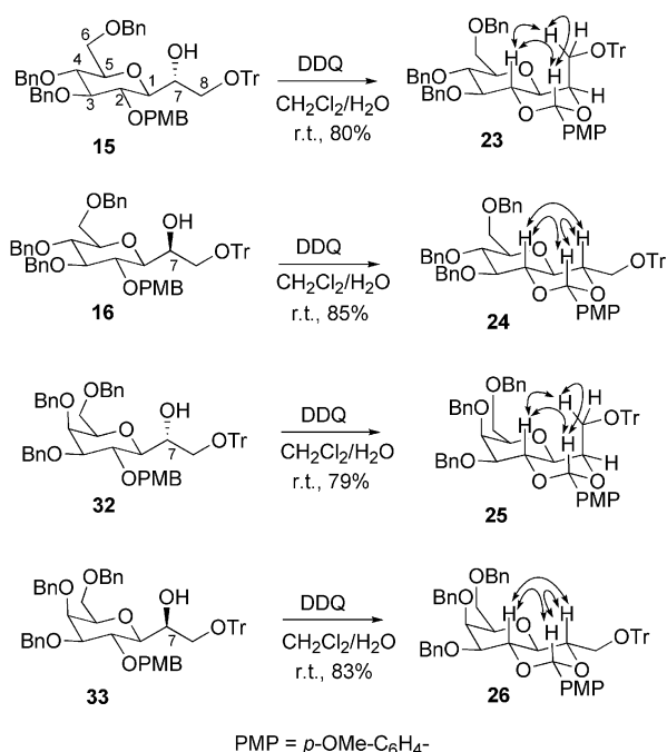
Scheme 2. Diagnostic nOe correlations for compounds 23 , 24 , 25 and 26 .
